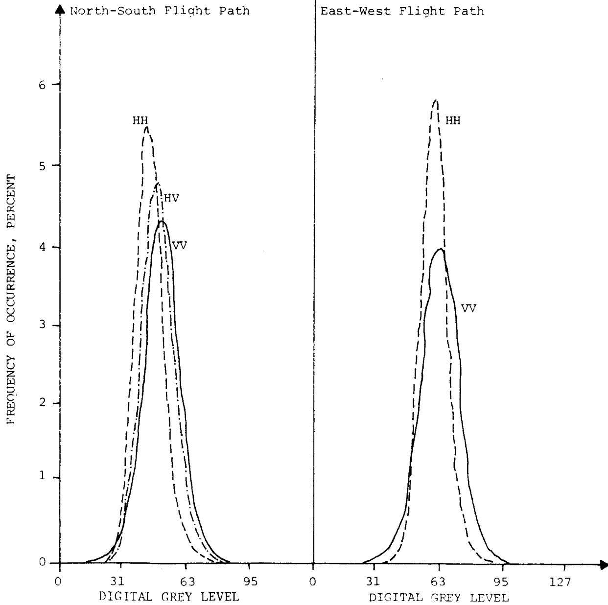
Figure 13. Histograms of SAR Data from Dade County
