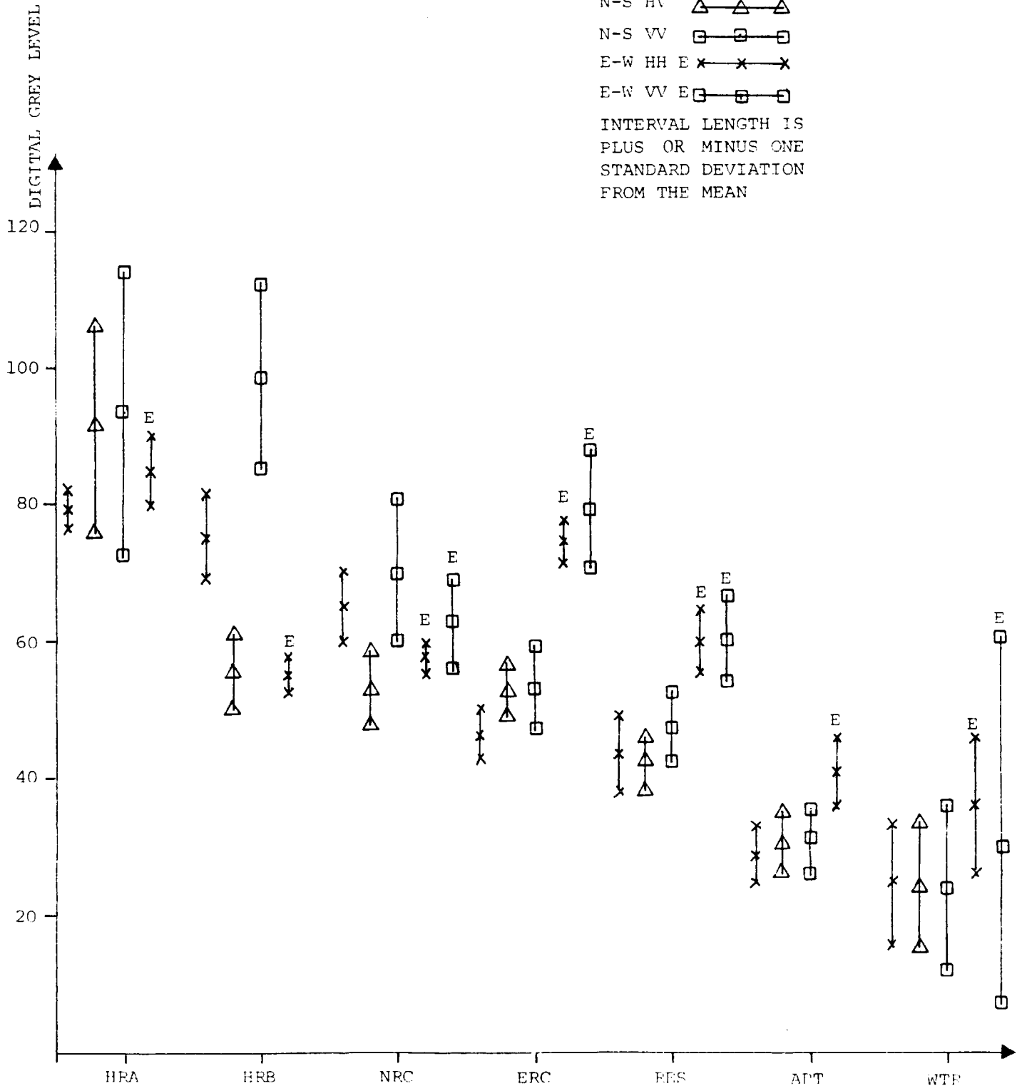
Figure 14. Means and Standard Deviations of Seven Land Cover Types from Dale County
